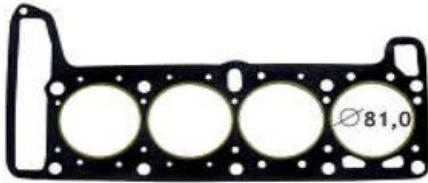
97001 SC - 1,8 MM - CIL. 81 MM 97001-KT - 3,0 MM - CIL. 81 MM 97001 TB - 2,3 MM - CIL. 81 MM JTA CABEÇOTE
